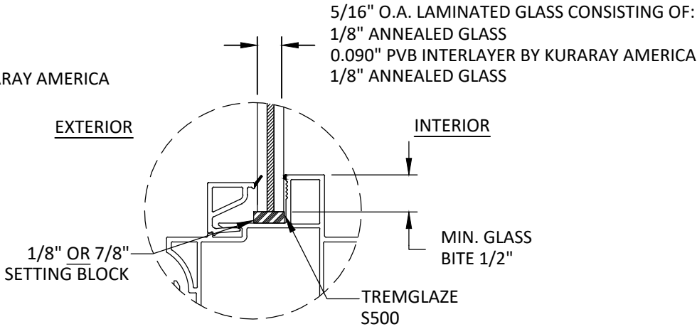
GLAZING DETAIL 2
