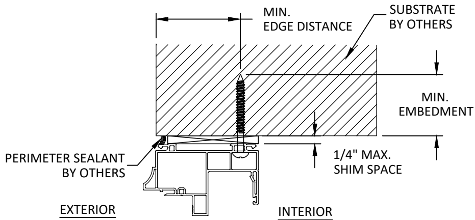
A 5 ANCHOR DETAIL THROUGH FRAME (HEAD)
