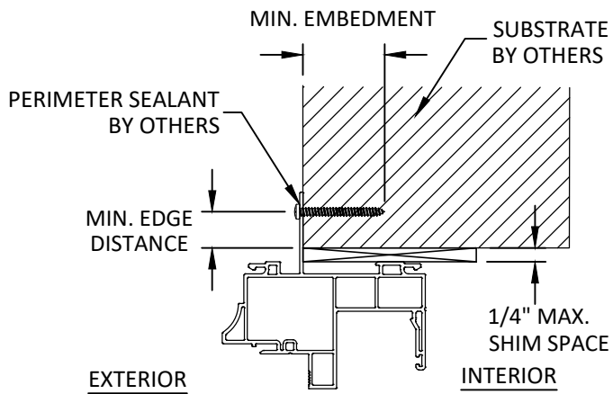
C 5 ANCHOR DETAIL NAIL FIN (HEAD)
