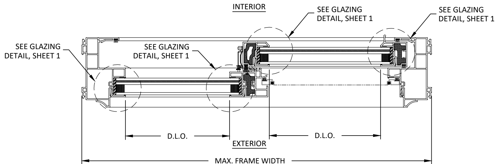
D 4 HORIZONTAL SECTION THROUGH FRAME
